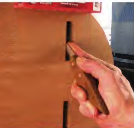
Marked in place. The tenons are marked directly from the mortises, ensuring that the locations match.
